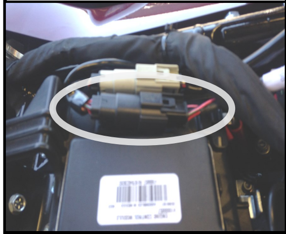
Harness Connector Location—on top of ECM
